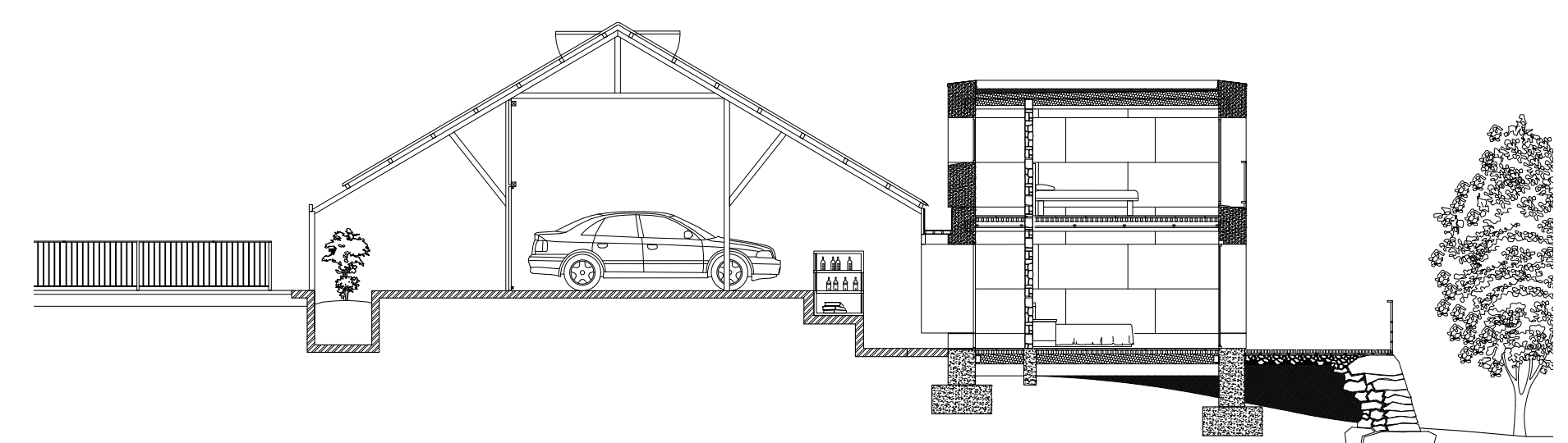
COUPE "NUIT"
