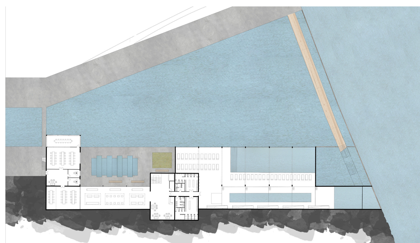
PLAN R-2
