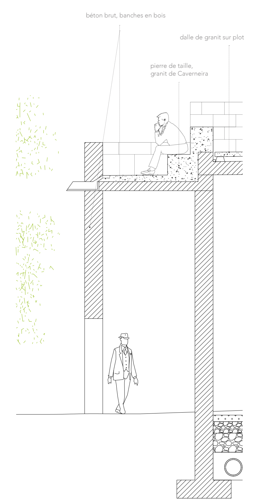
COUPE DETAIL, PAVILLON DE MEDITATION, 1.50e
