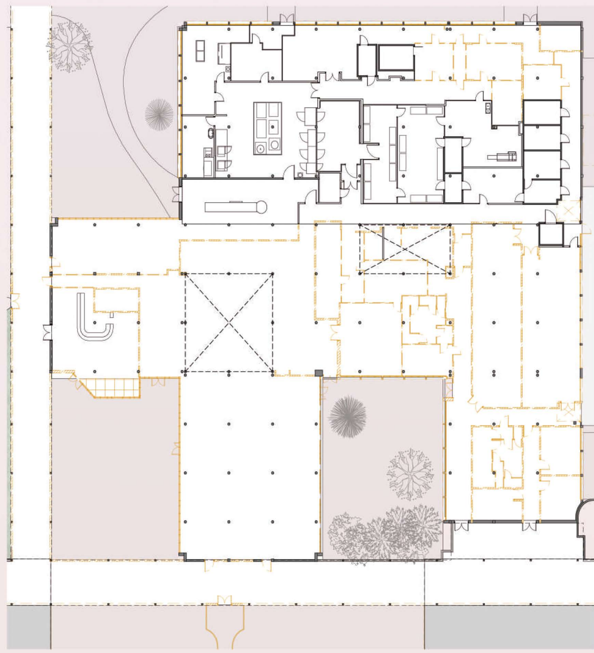
PLAN - DECONSTRUCTION
