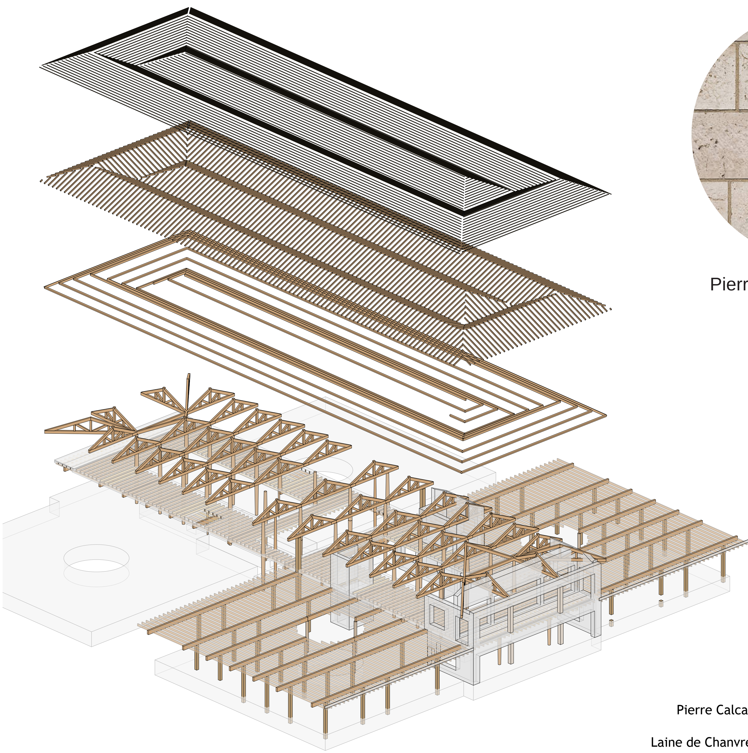
Structure bois
