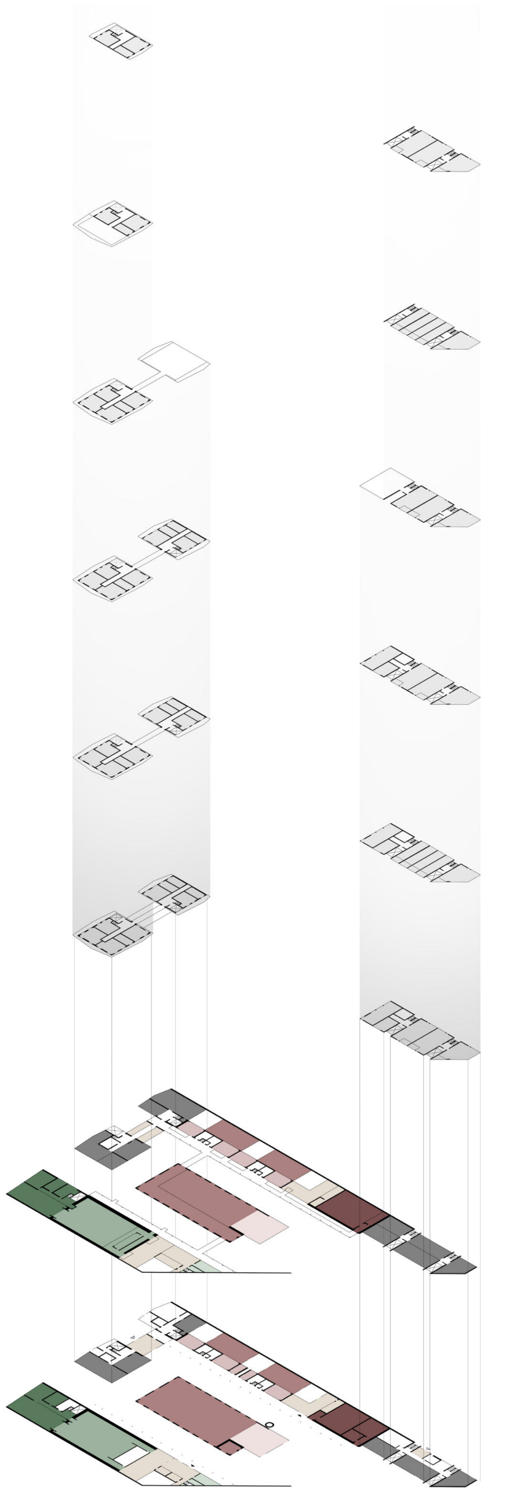
ORGANIGRAMME
