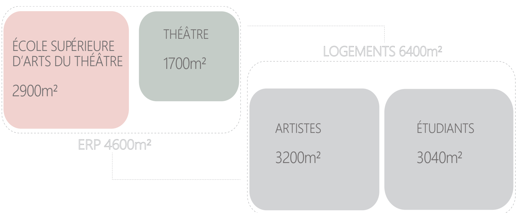
ORGANIGRAMME
