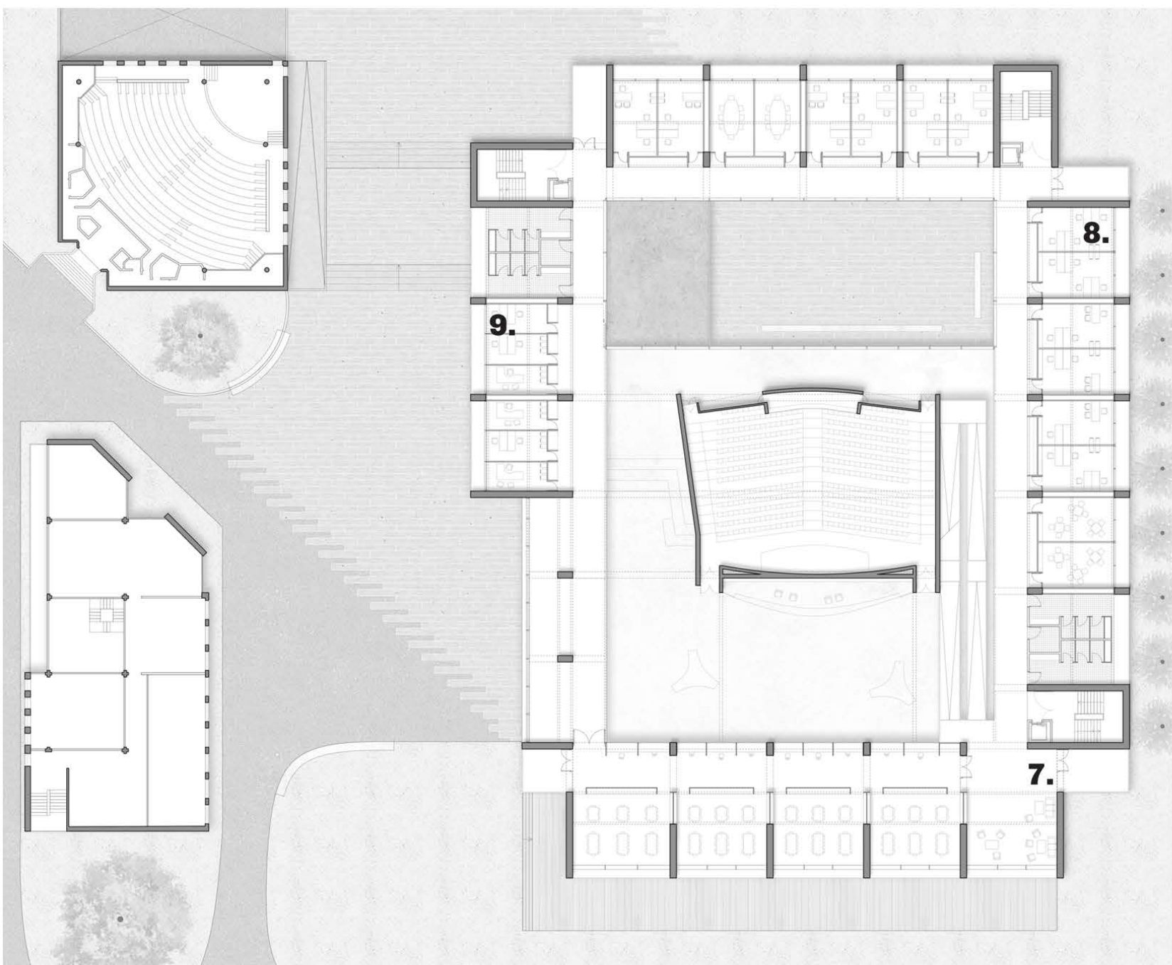
FIRST FLOOR 1 : 500
