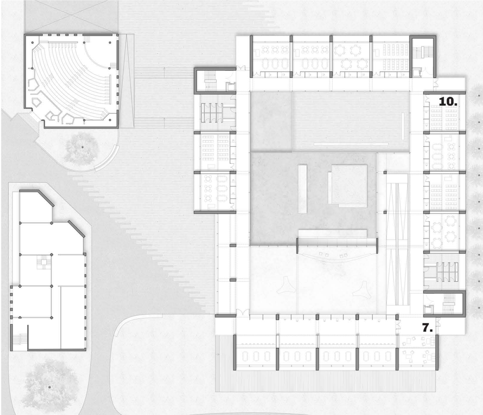
SECOND FLOOR 1 : 500
