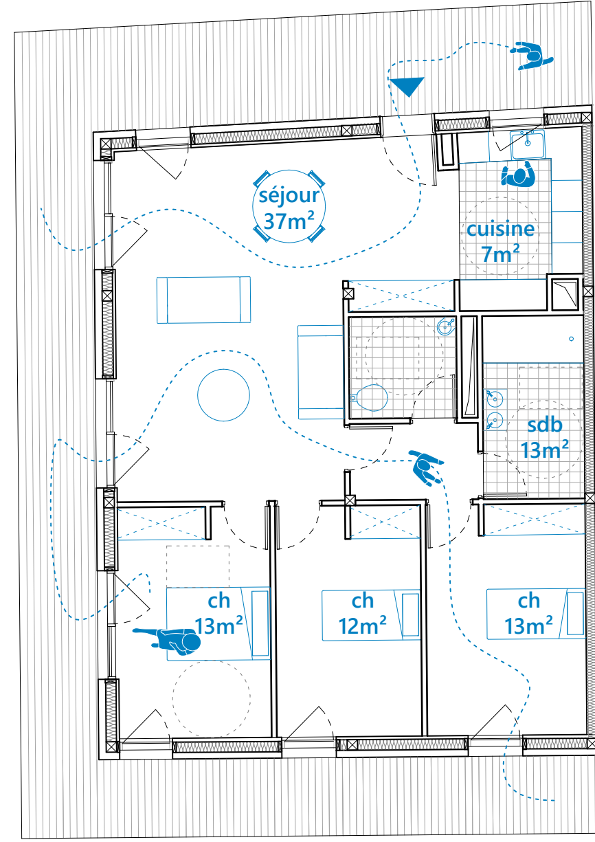
PLAN T4 100m 2 1/100
