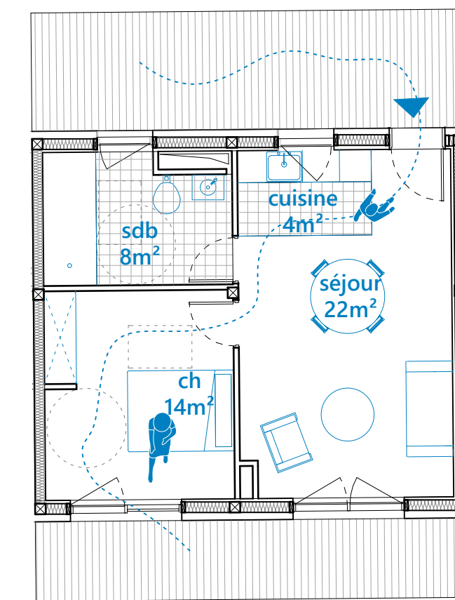
PLAN T2 50m 2 1/100
