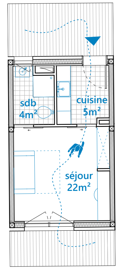
PLAN T1 26m 2 1/100
