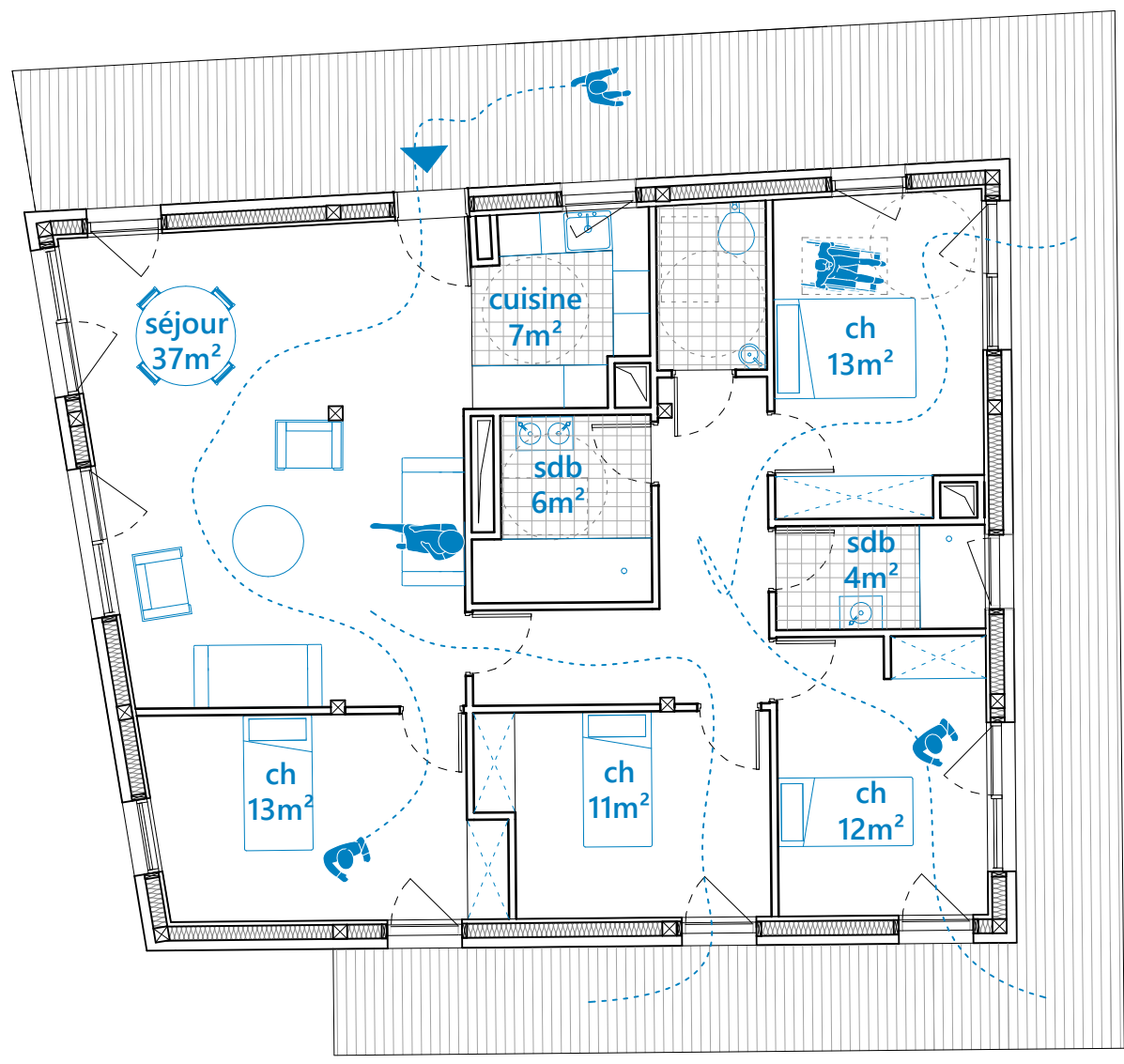
PLAN T5 120 m 2 1/100
