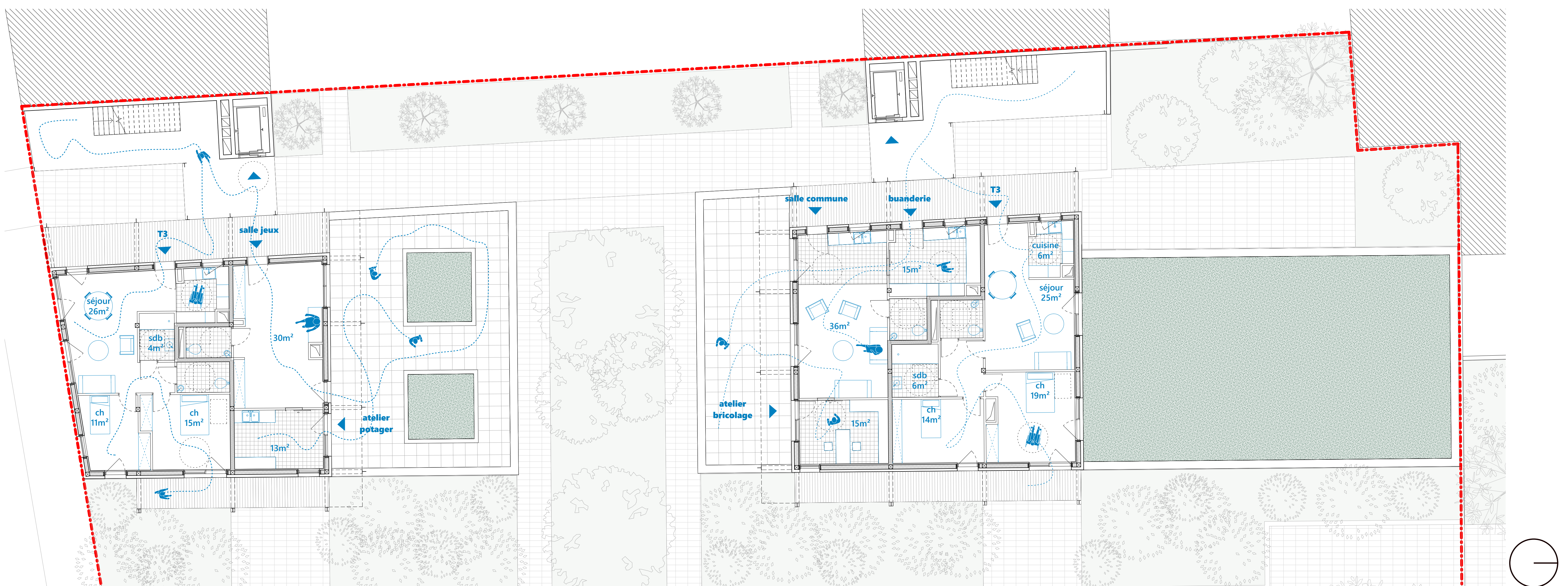
PLAN R+1 1/100
